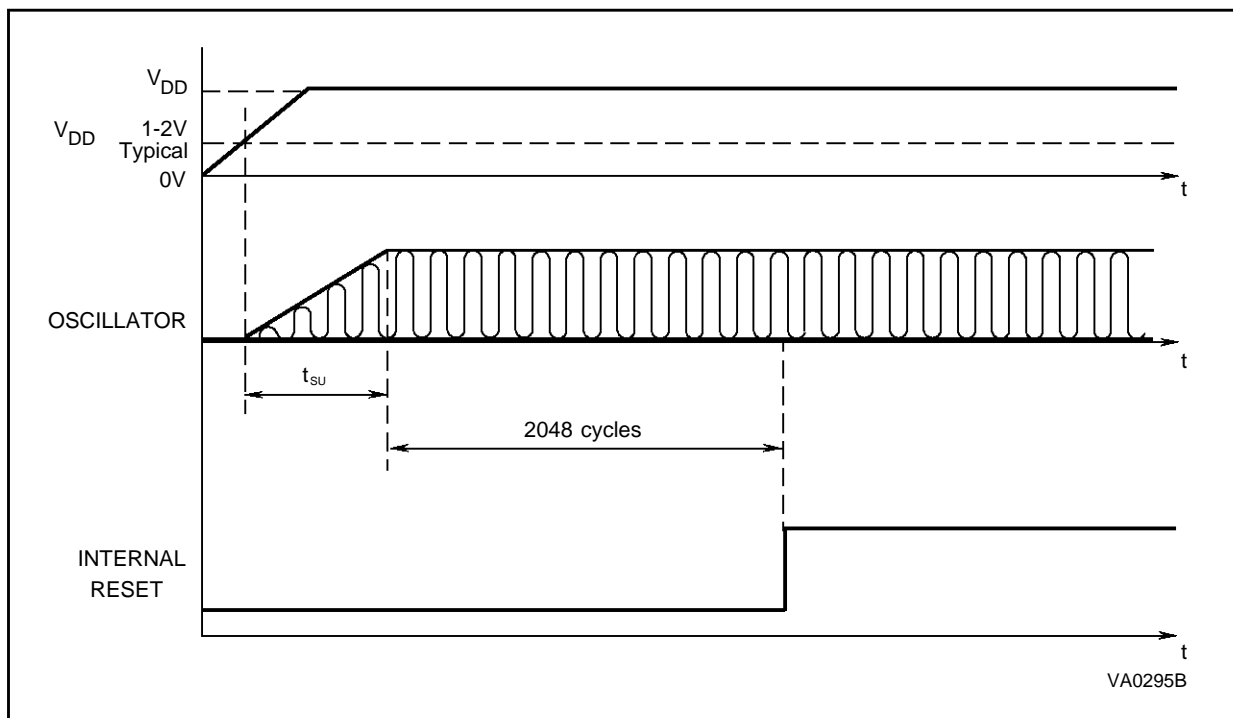
Figure 30. Power-on-Reset
