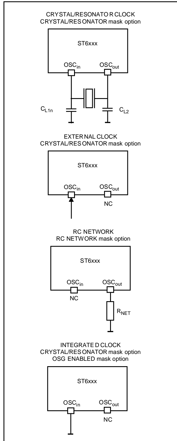
Figure 11. Oscillator Configurations
